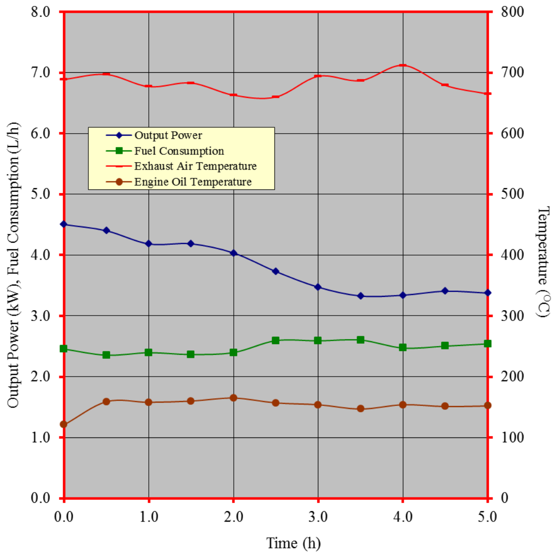
Figure 4. Performance characteristic curves during the continuous running test of the KENBO KB7.5M gasoline engine
