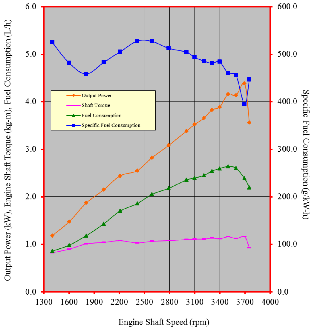
Figure 3. Performance characteristic curves of the KENBO KB7.5M gasoline engine
